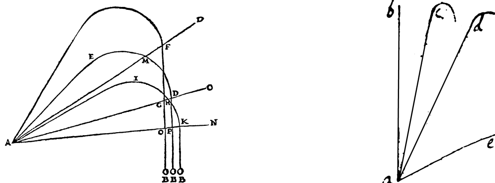
Figure 7. COMPARISON OF TARTAGLIA'S CONSTRUCTION OF PROJECTILE TRAJECTORIES (LEFT FIGURE) WITH GALILEO'S FIGURE IN De Motu (RIGHT FIGURE) 30
