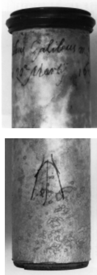
Figure 9. ALLEGORICAL DRAWING OF GALILEO ON THE TUBE OF A TELESCOPE TOGETHER WITH A TEXT INCLUDING THE DATE MARCH 20, 1629. THE DRAWING REPRESENTS HIS DISCOVERY OF THE PARABOLIC SHAPE OF THE PROJECTILE TRAJECTORY, ACCOMPANIED BY THE DATE MARCH 20, 1629. ORIGINALLY, DRAWING AND TEXT BELONGED PROBABLY TO AN ENTRY IN AN “ALBUM AMOCORUM” AND WERE LATER ATTACHED TO THE TELESCOPE IN ORDER TO PRETEND THAT IT IS A UNIQUE AND VALUABLE INSTRUMENT. 38
