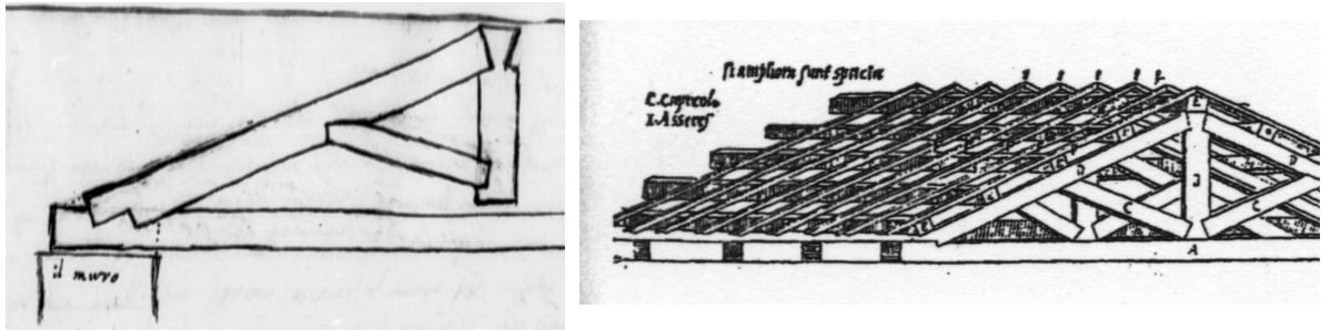
Figure 5. GUIDOBALDO'S SKETCH AND A CONTEMPORARY REPRESENTATION OF A ROOF WITH "CAPRIATA". 23
