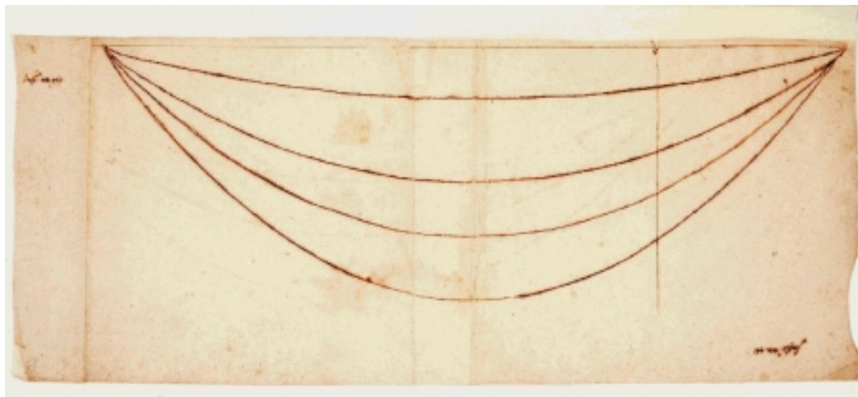
Figure 1. Ms. GAL. 72, FOLIO 41/42 WITH CURVES PRODUCED BY MEANS OF A HANGING CHAIN
